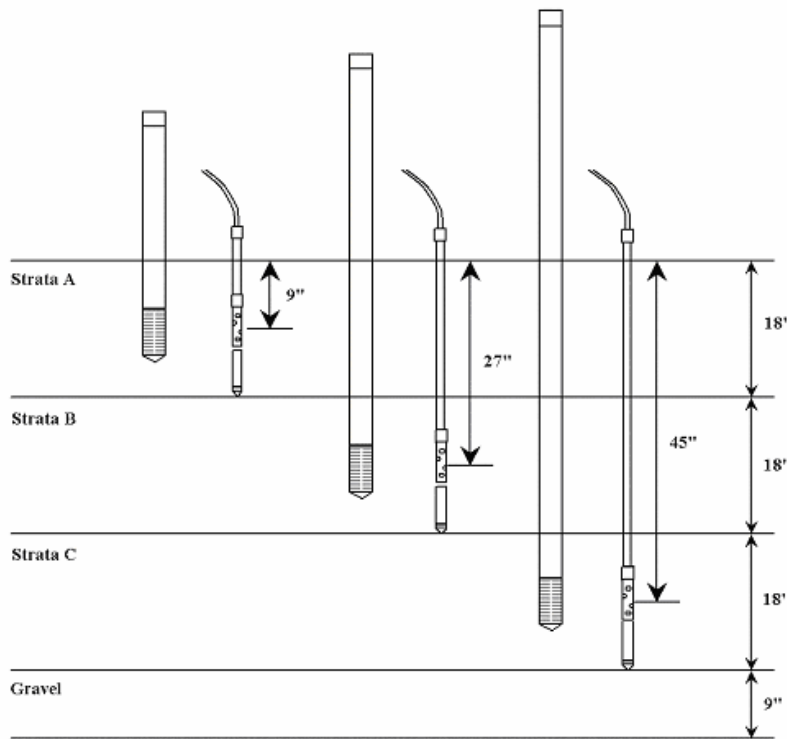
Figure 5. Peizometer & well cross-sections showing the placement of screened area at the center of each stratum
